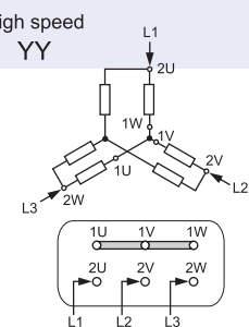
Centrifugal drive, Dahlander connection
